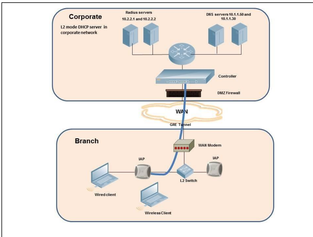
Figure 137 Scenario 4 - GRE: Single Datacenter Deployment with No Redundancy
